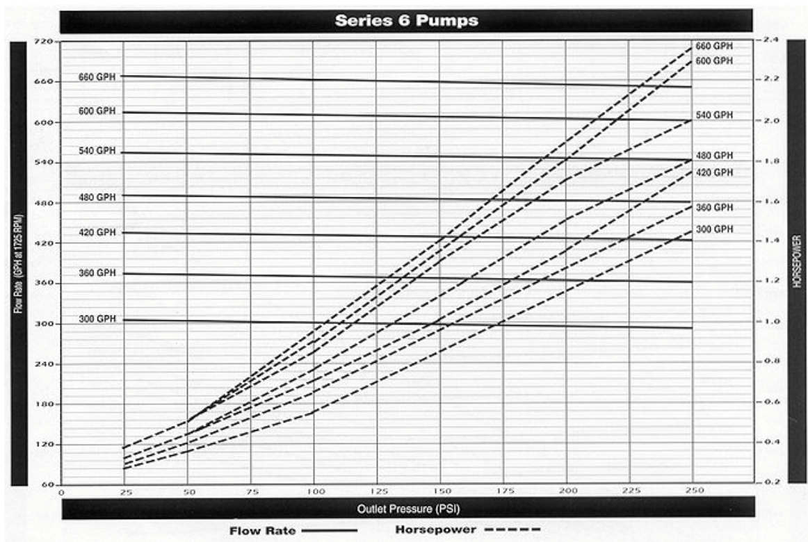
Capacities & Horsepower Graph
