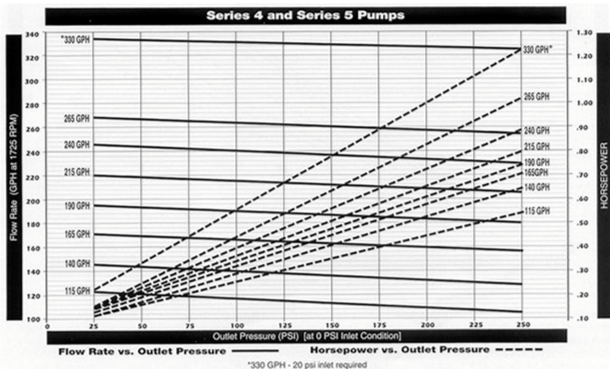
Capacities & Horsepower Graph
